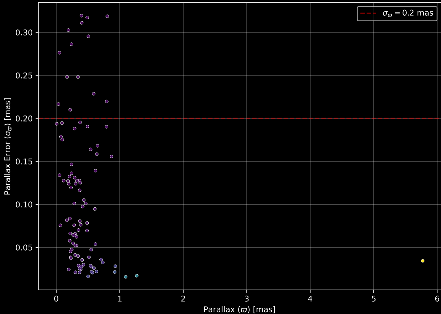
APOGEE DR17 Field: [005+00] Parallax Quality (n= 96)
