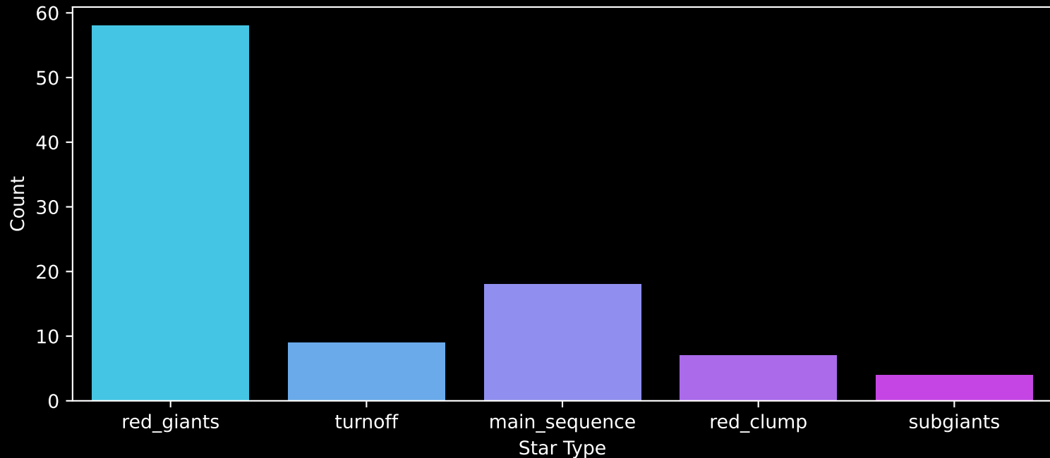
APOGEE DR17 Field: [005+00] Count plot of Star Type
