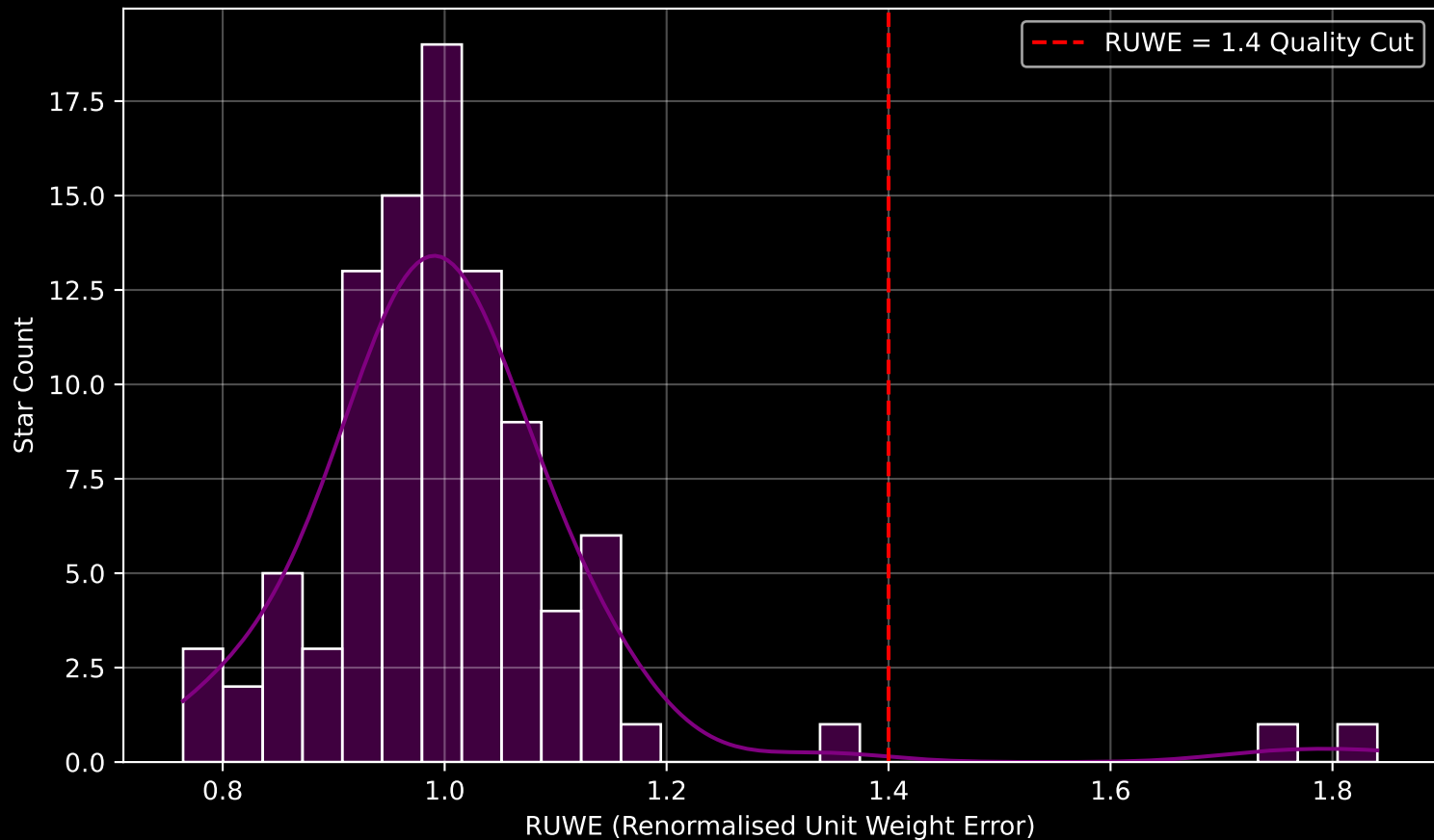
GAPOGEE DR17 Field [005+00] RUWE Distribution (n= 96)
