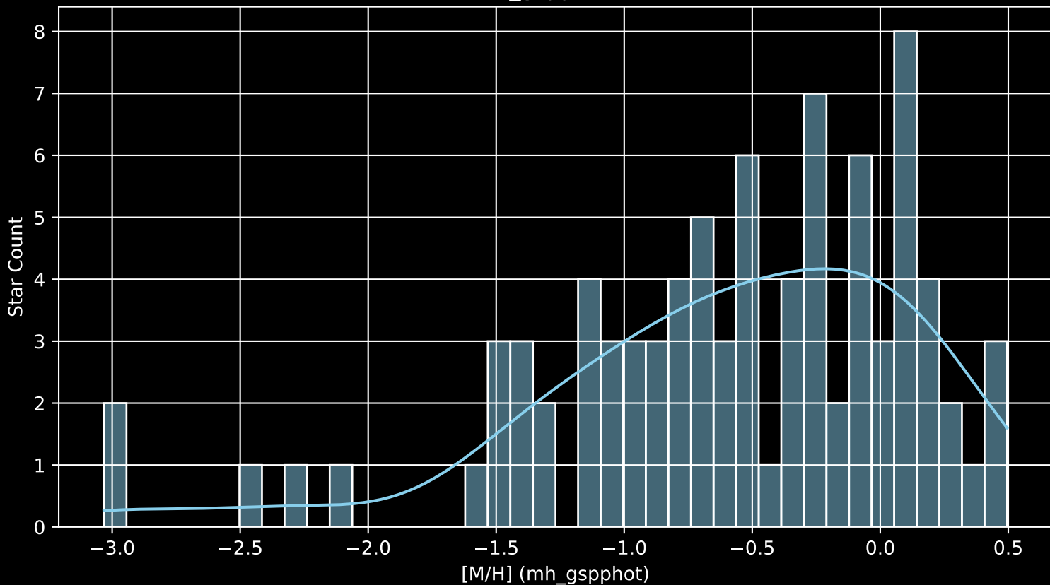
APOGEE DR17 Field: [005+00] [M/H] (mh_gspphot) (n= 86)
