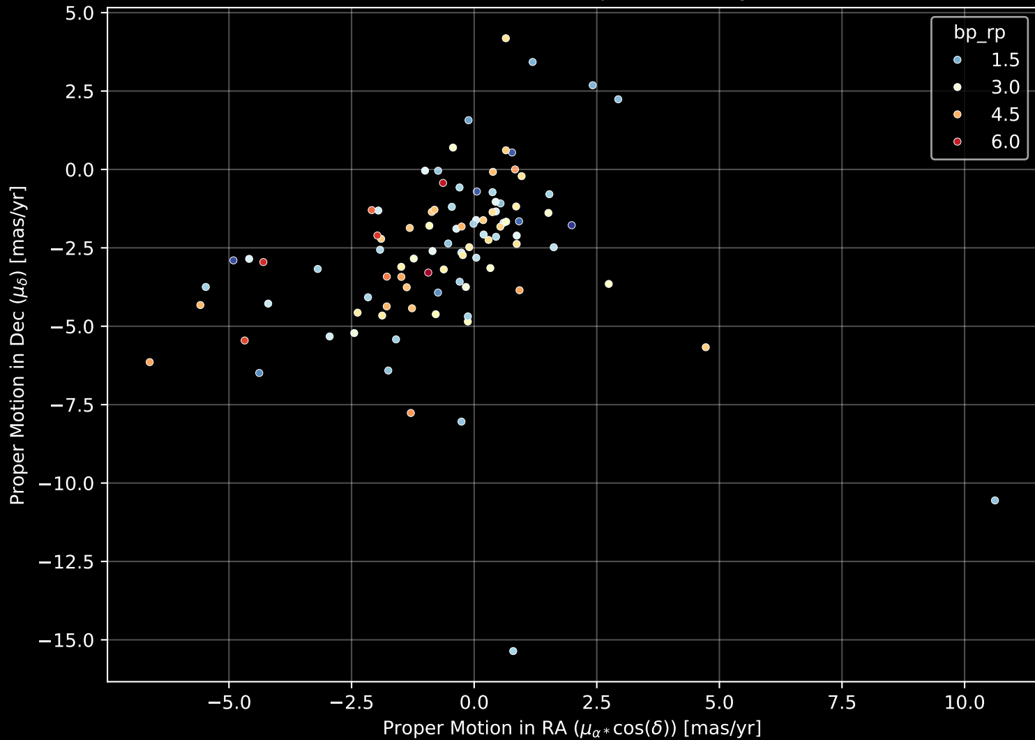
APOGEE DR17 Field: [005+00] Proper Motion Diagram (n= 96)
